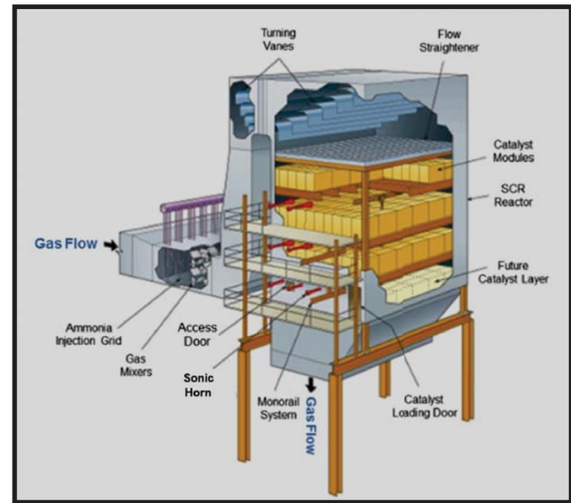
Squared Inlet Roof
